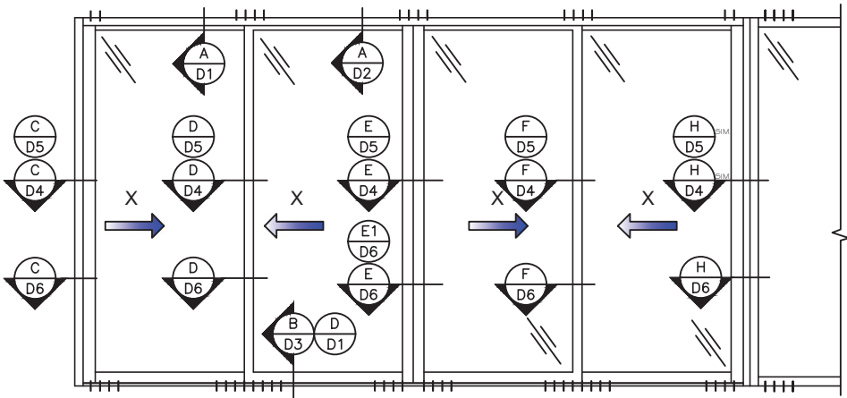
(4) PANELS SGD XXXX NO WATER RESISTANCE
