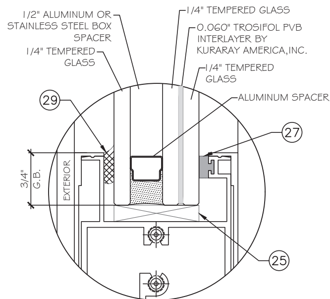
GLASS TYPE "G2" 1 5/16" INSULATED LAMINATED GLASS LAMINATED ON INTERIOR SIDE
