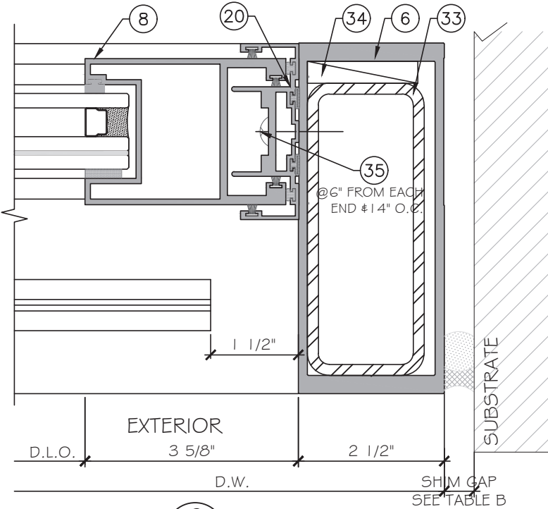
G D5 DETAIL
