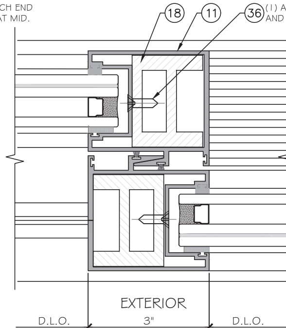
D D4 DETAIL
