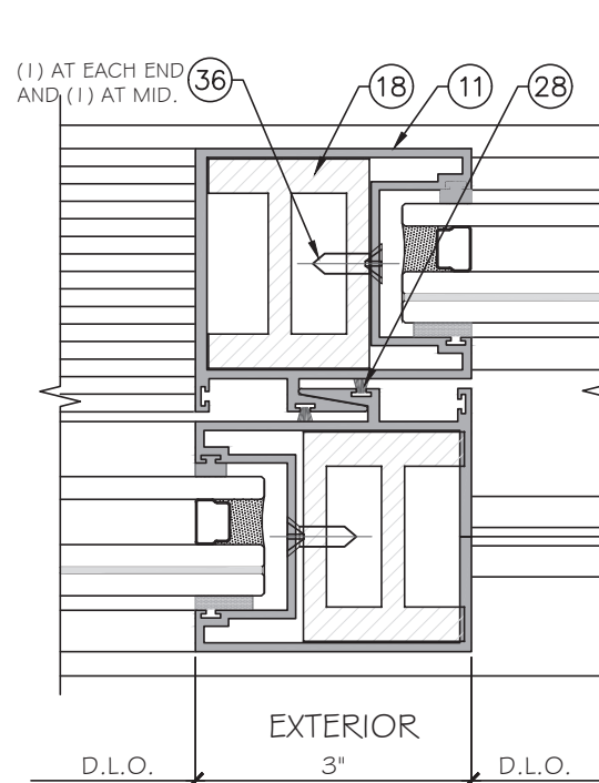
C D4 DETAIL
