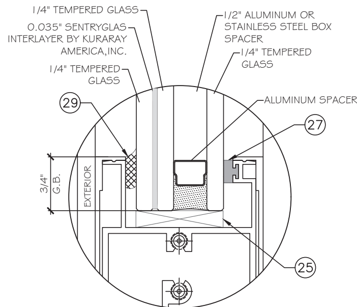
GLASS TYPE "G3A" 1 5/16" INSULATED LAMINATED GLASS LAMINATED ON EXTERIOR SIDE
