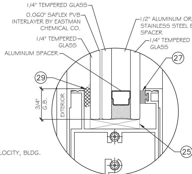
GLASS TYPE "G4A" 1 5/16" INSULATED LAMINATED GLASS LAMINATED ON EXTERIOR SIDE
