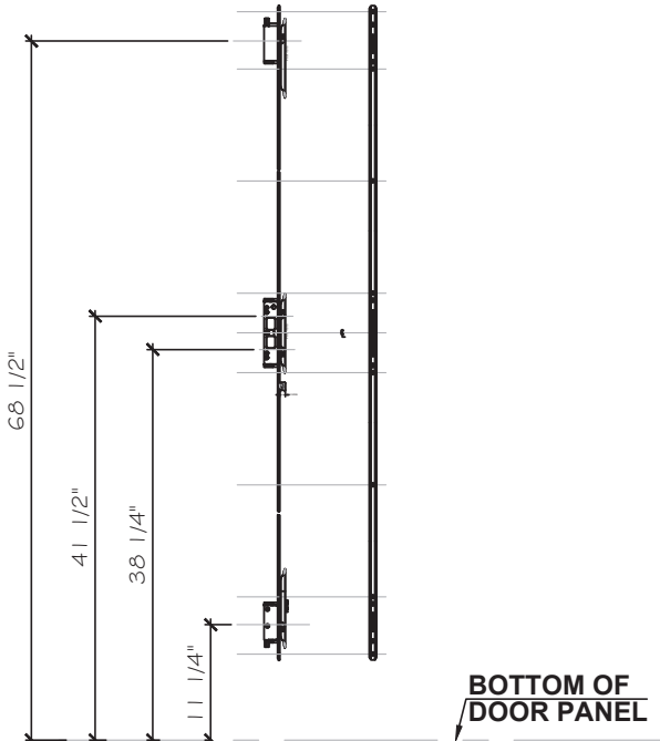
LOCK POINTS LAYOUT.
