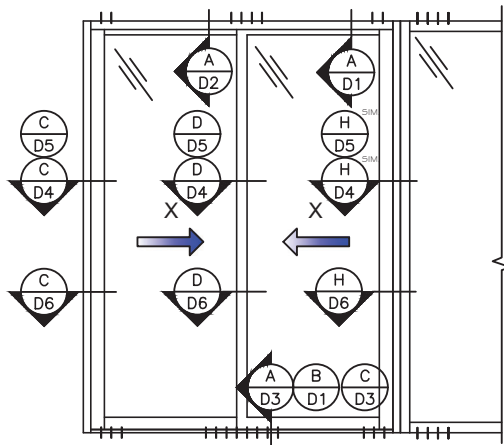
(2) PANELS SGD XX NO WATER RESISTANCE
