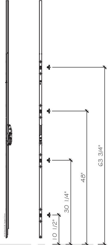
LOCK POINTS LAYOUT FOR 10'-0" DOOR HEIGHT AND 12'-6" DOOR HEIGHT. (LIFT & SLIDE DOOR)
