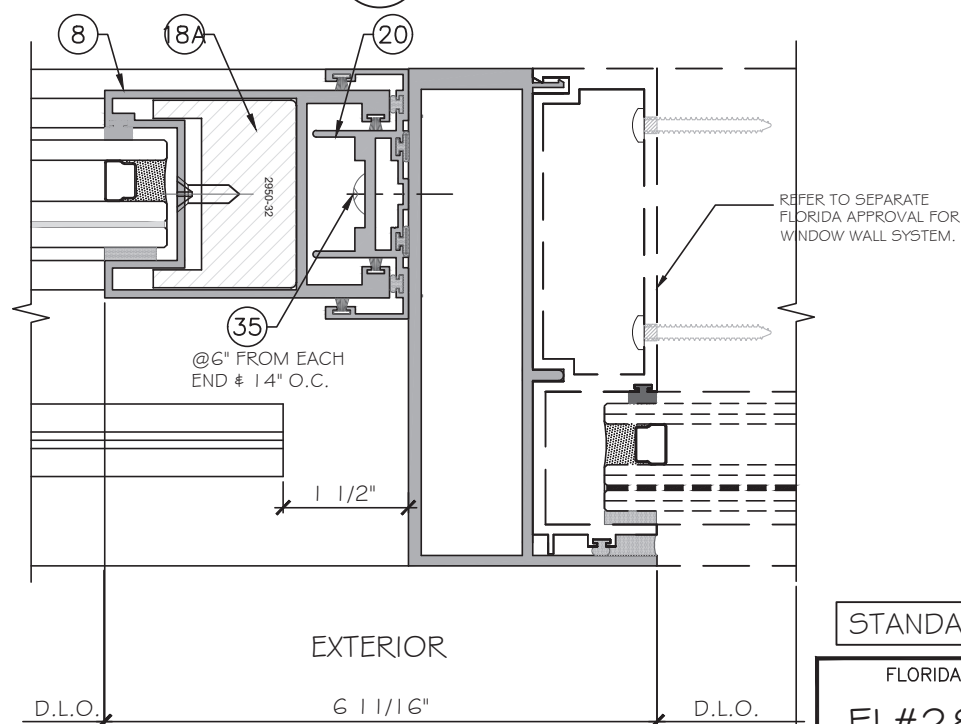
H D6 DETAIL
