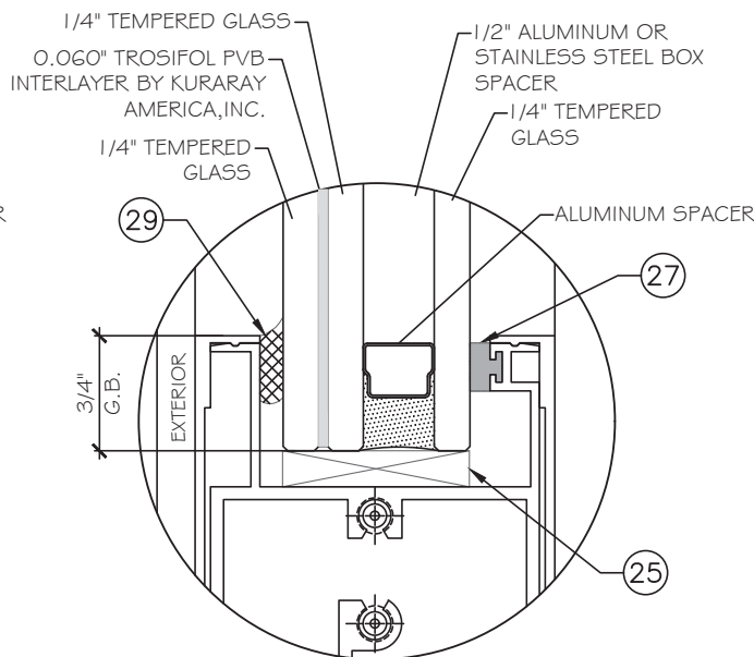
GLASS TYPE "G2A" 1 5/16" INSULATED LAMINATED GLASS LAMINATED ON EXTERIOR SIDE
